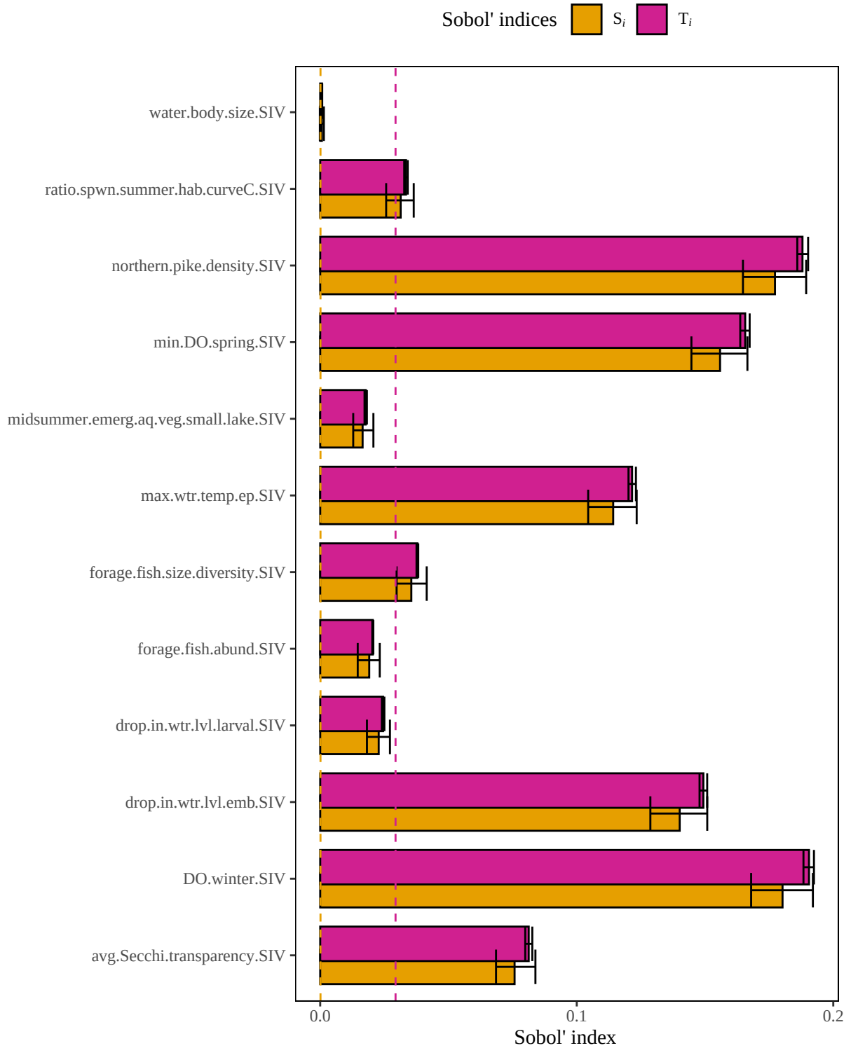
Figure 5. Results of a sensitivity analysis for the muskellungeSmallLakeSpwnVegCurveC model based on a geometric mean structure. Dashed lines represent baseline numerical approximation error for S_i and T_i ( i.e. , dummy variables).
